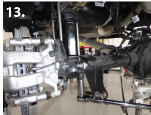
11. Install lift blocks and new U-bolts. Torque to 95 ft.lbs. (pic 13)
